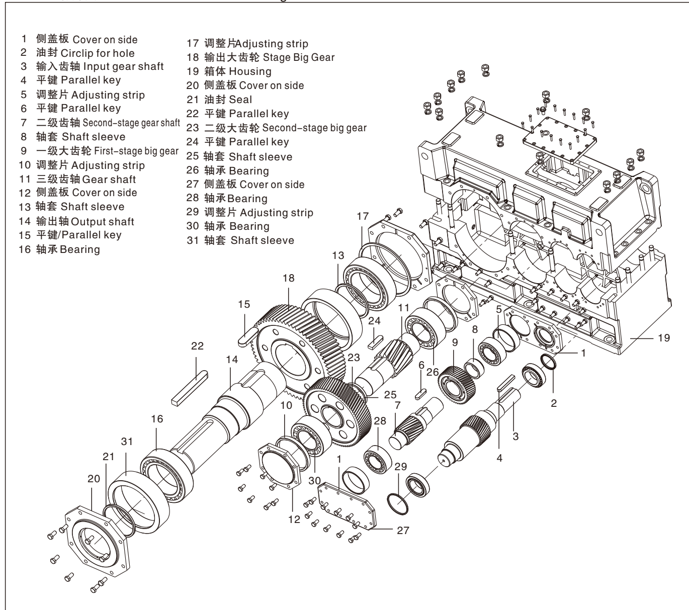
WH系列结构图:/WH series structure drawing:
