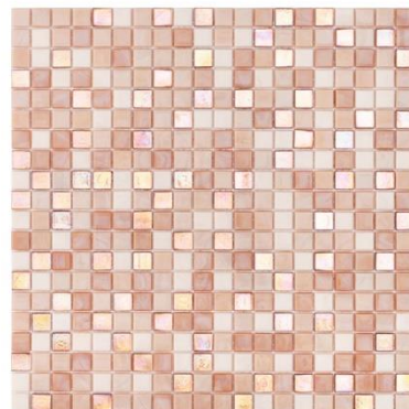
Fired Earth Glass 15mm Mixed 327mm*327mm Thickness: 4mm
