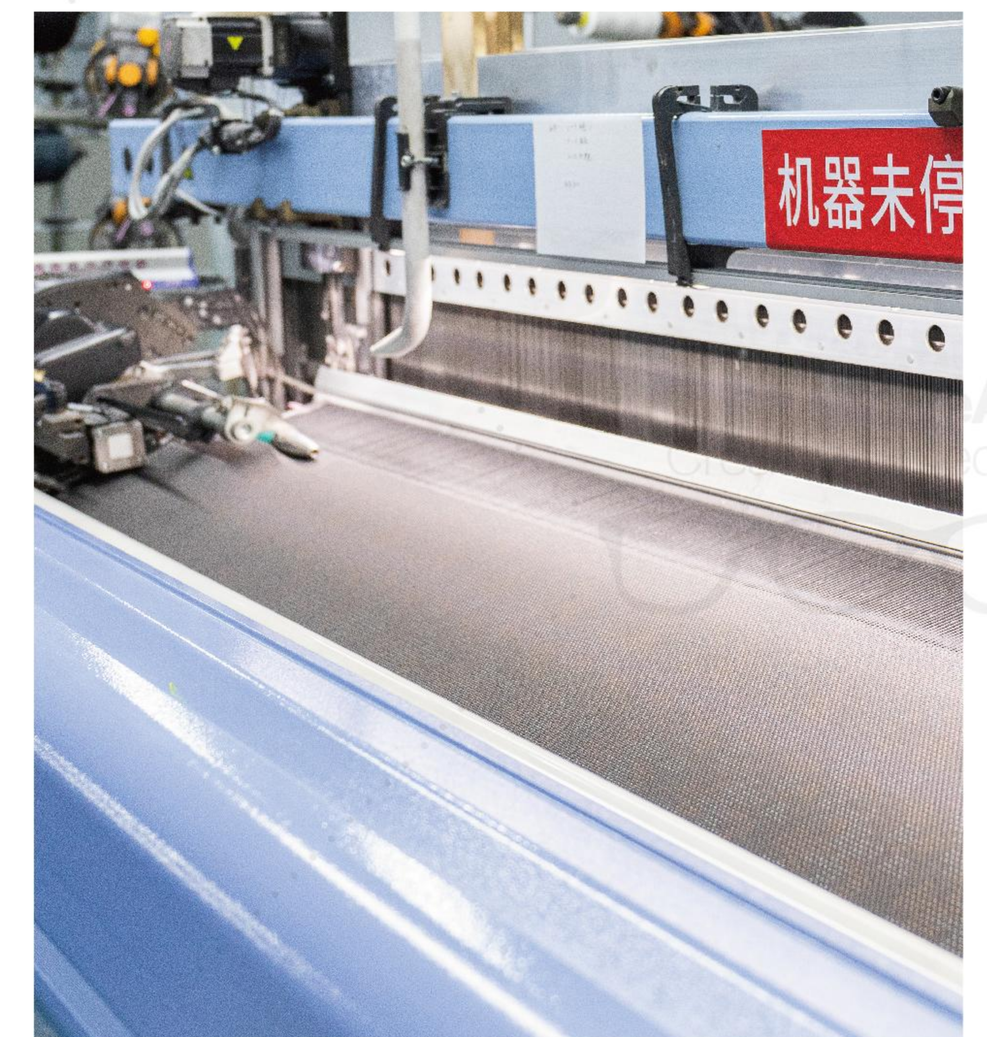
剑杆机 Rapier Weaving Machine
