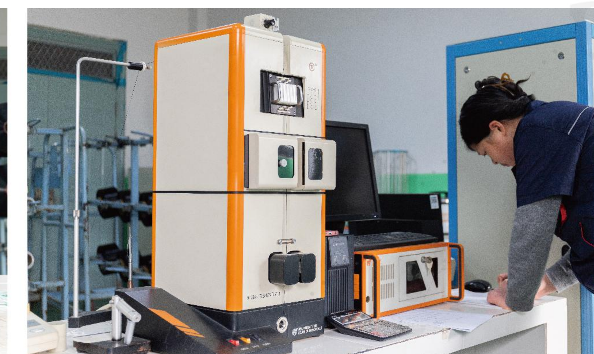
条干仪 Evenness Tester
