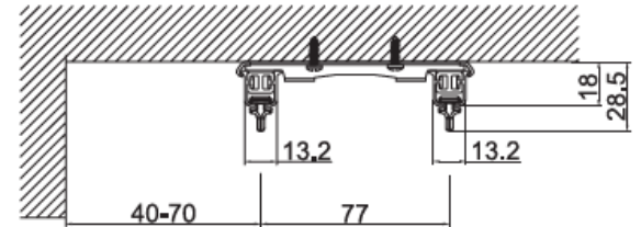
Mount on wall - single track instruction
