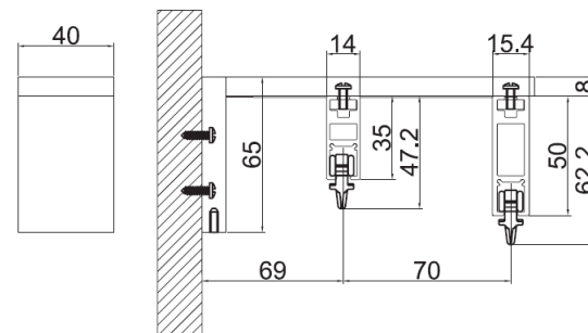
Mount on wall - double track instruction
