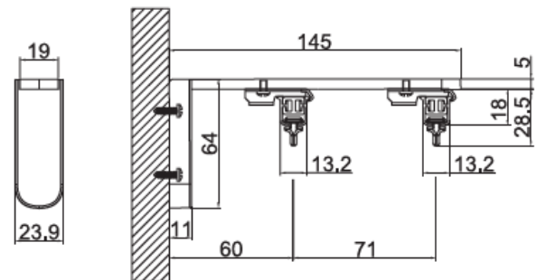
Mount on wall - double track instruction
