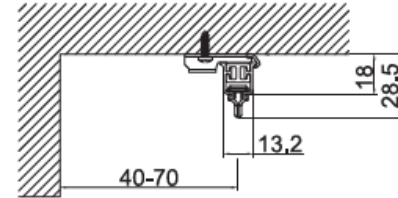
Mount on ceiling - double track instruction
