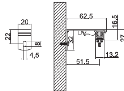
Mount on wall - double track instruction
