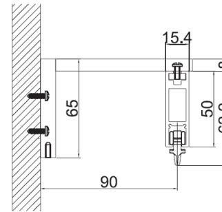
Mount on wall - double track instruction
