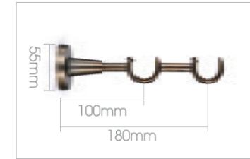
Double Track Wall Bracket
