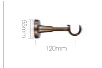
Single Track Wall Bracket
