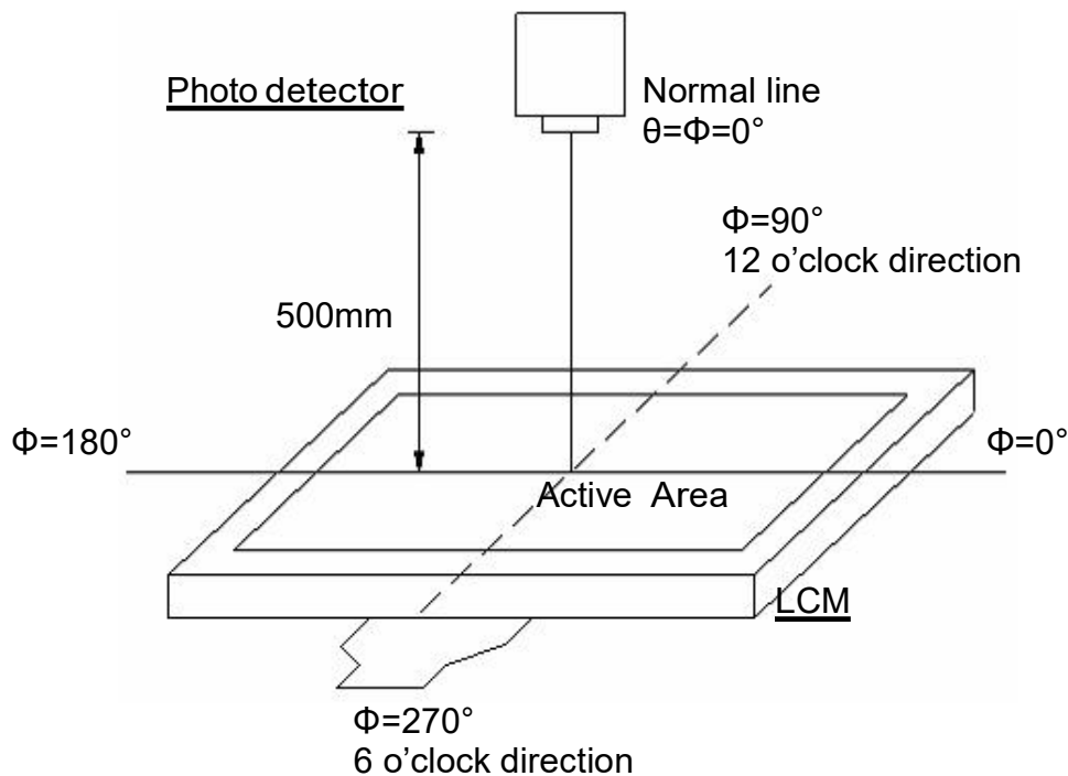
Fig. 4-2 Optical measurement system setu
