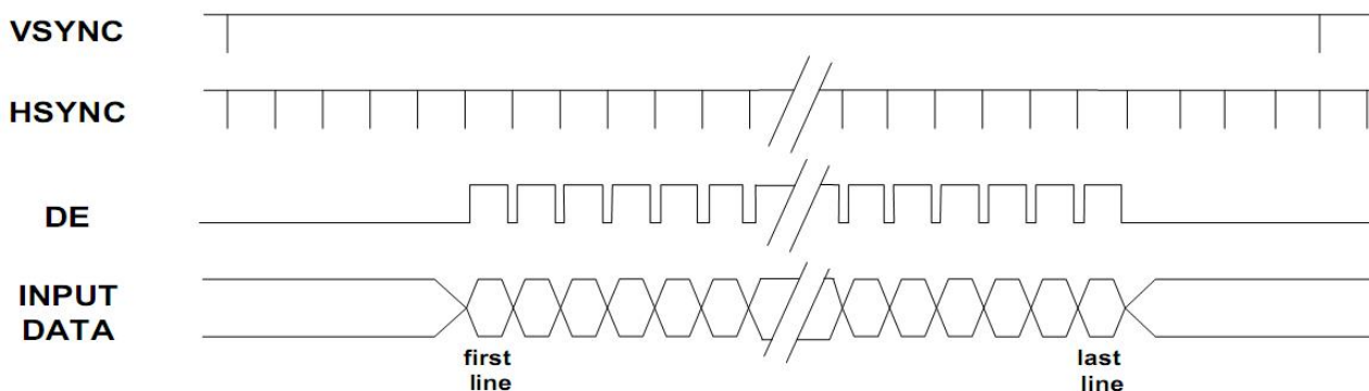
Vertical Input Timing
