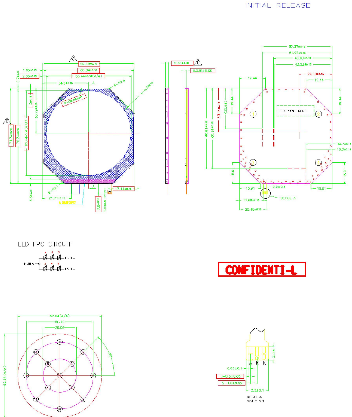
Figure 6. BLU Outline Dimension (unit: mm)
