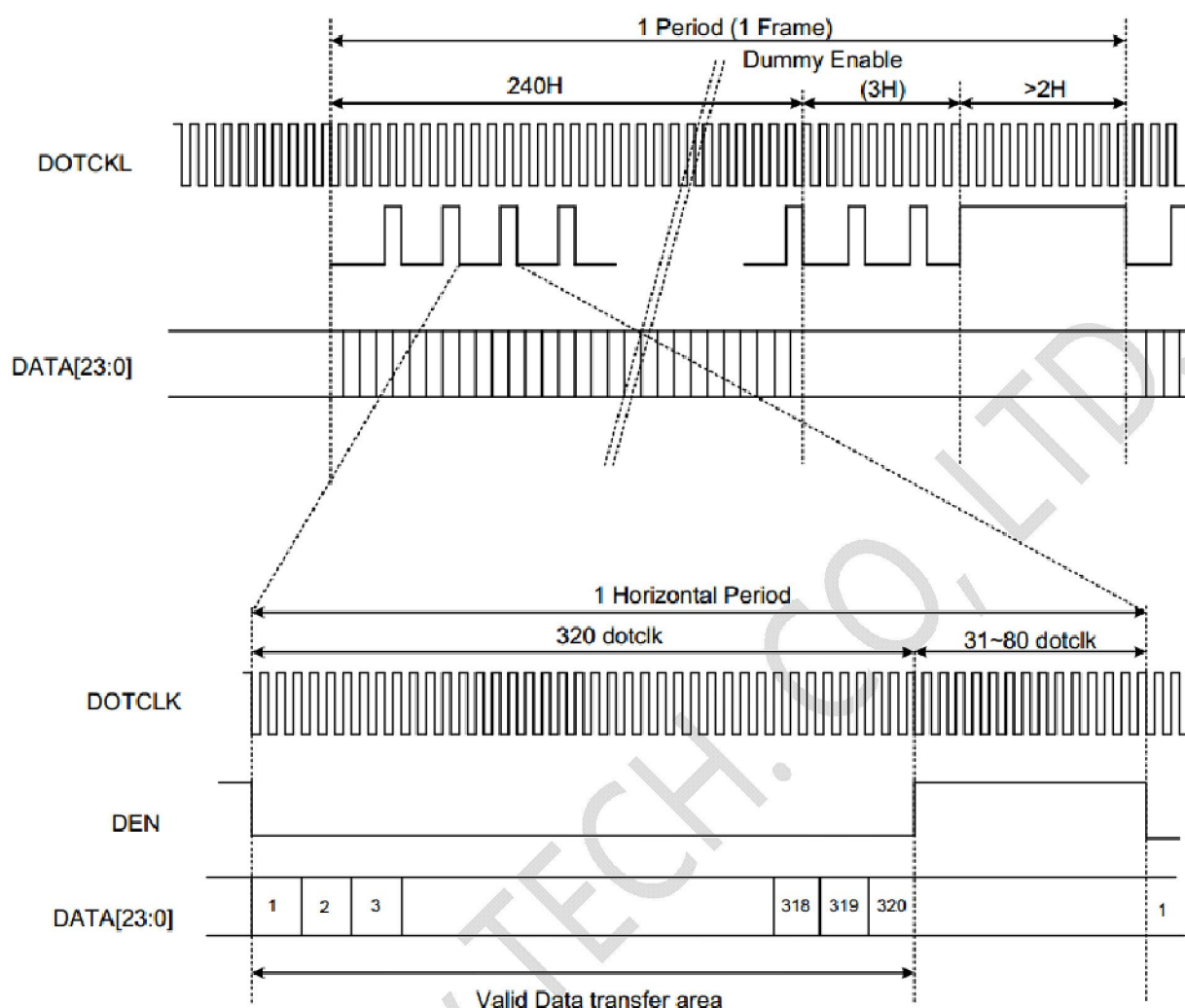
Figure Signal Timing in DE Mode
