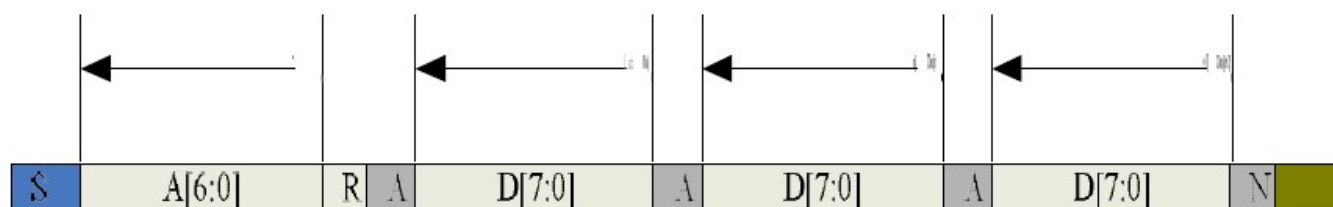
IIC master read, slave write
