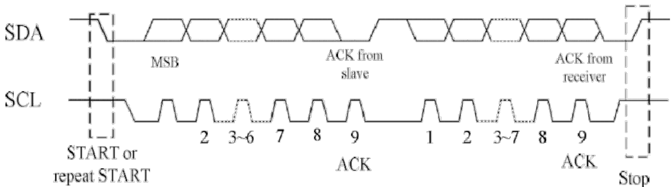
IIC Serial Data Transfer Format
