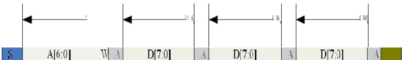
IIC master write, slave read
