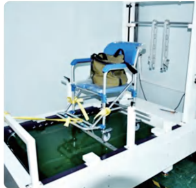
ROAD RUNNING TEST MACHINE
