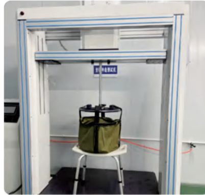
SEAT IMPACT TESTING MACHINE
