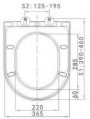
BF-JX073 Size: 445x365x35mm Adjustable distance: S1:390-460 / S2:125-195
