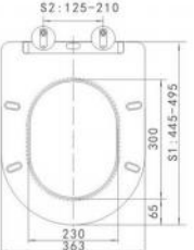
BF-JX085 Size: 455x363x40mm Adjustable distance: S1:445-495 / S2:125-210
