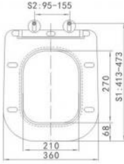
BF-JX118 Size: 435x360x50mm Adjustable distance: S1:413-473 / S2:95-155
