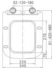
BF-JX043 Size: 460x345x60mm Adjustable distance: S1:420-480 / S2:120-180
