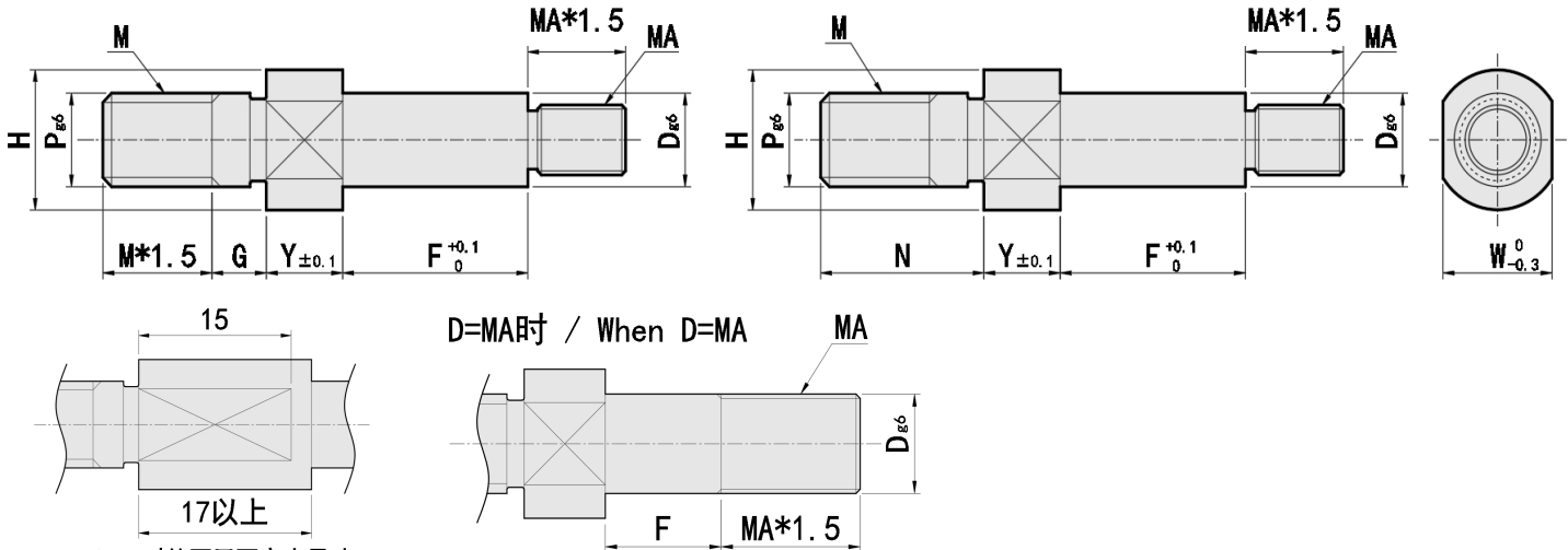
Y≥17时的两平面宽度尺寸 Dimensions of Wrench Flats when Y≥17
