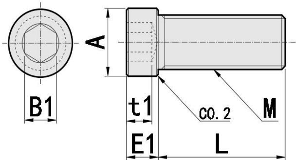
短头型小径螺栓/Low Small Head Cap Screws ZKBB / ZKBBS
