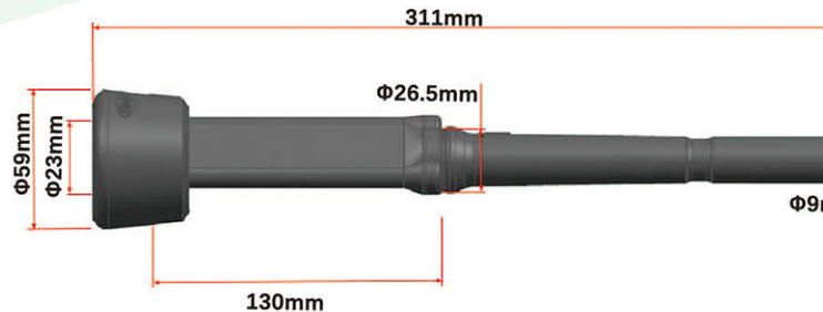
IP10S without air outlet YH-ME105A Material:Rubber
