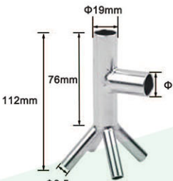
YH-ME231 S.S. distributor
