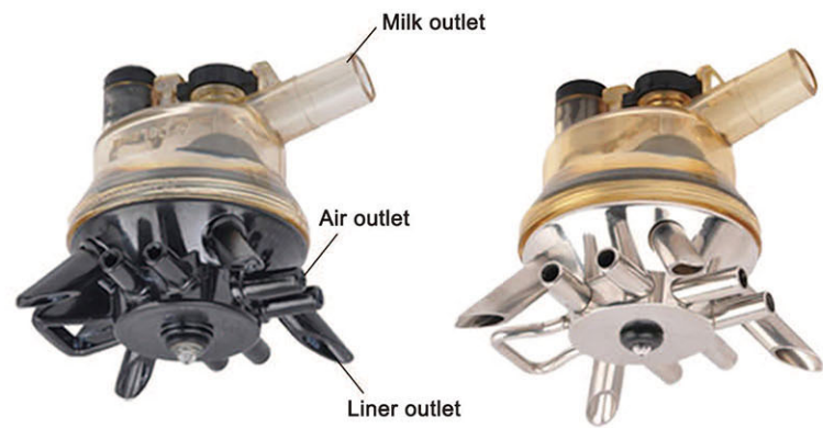
MC11 Milk Claw
