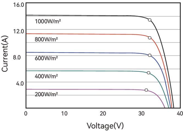
I-V Curves of PV Module (440W)
