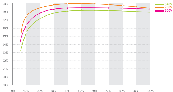
MAX 80KTL3 LV efficiency
