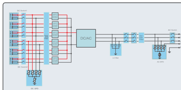
MAX 50-80k TL3 LV topology
