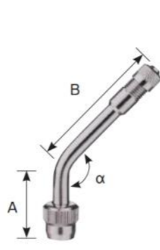
JT36M-135°
