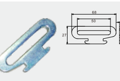
BTFTH010 TRACK FITTING CAP: 1,250 kgs / 2,750 lbs.
