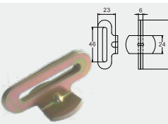
BTFTH007 BUTTERFLY FITTING FOR 25MM HOLE CAP: 909 kgs / 2,000 lb.
