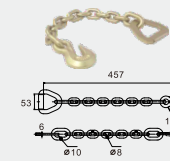
BTCA002 18" CHAIN ANCHOR W/ 2" DELTA RING, WEAR PAD CAP: 5,454 kps./ 12,010 lbs.
