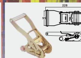
BTRB021 2" WITH ALUM LONG WIDE HANDLE CAP: 6,000 kgs / 13,200 lbs.
