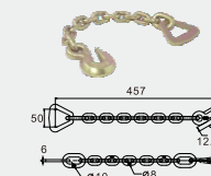
BTCA001 16" CHAIN ANCHOR W/ 2" DELTA RING CAP: 5,454 lbs./ 12,000 lbs.
