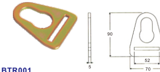
BTR001 2" FLAT DELTA RING CAP: 6,000 kgs / 13,200 lbs.
