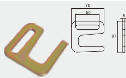
BTFTH002 2" SLAT HOOK CAP: 1,363 kgs / 3,000 lbs.
