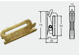
BTFTH008 SPRING LOADED FITTING CAP: 2,727 kgs / 6,000 lbs.
