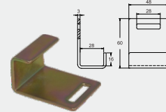
BTSF005 1" FLAT HOOK CAP: 1,000 kgs / 2,200 lbs.
