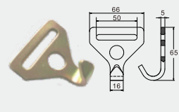
BTFTH001 2" F TRACK HOOK CAP: 1,000 kgs / 2,200 lbs.
