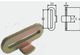
BTFTH006 BUTTERFLY FITTING FOR 19MM HOLE CAP: 680 kgs / 1,500 lbs.
