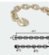
BTCA006 16" CHAIN ANCHOR W/ TUBE WELDED GAP: 5,454 kips / 12,000 lb
