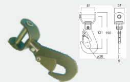
BTSF006 1-3/4" SWIVEL SNAP HOOK CAP: 3,500 kgs / 7,700 lbs.
