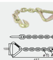
BTCA005 18" CHAINANCHOR W/ 4" FORGED RING CAP: 9,050 kgs / 20,000 lbs.
