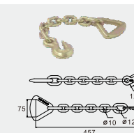
BTCA004 18" CHAIN ANCHOR W/ 3" FORGED RING CAP: 8,181 kg/ 18,000 lbs.
