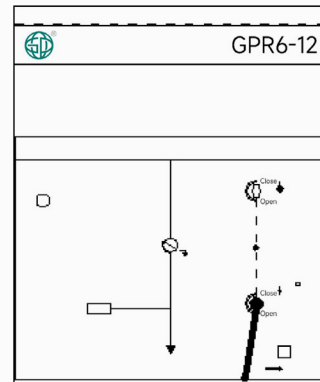
Schematic diagram of opening operation
