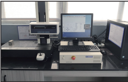
台式粗糙度仪 Desktop Roughness Tester
