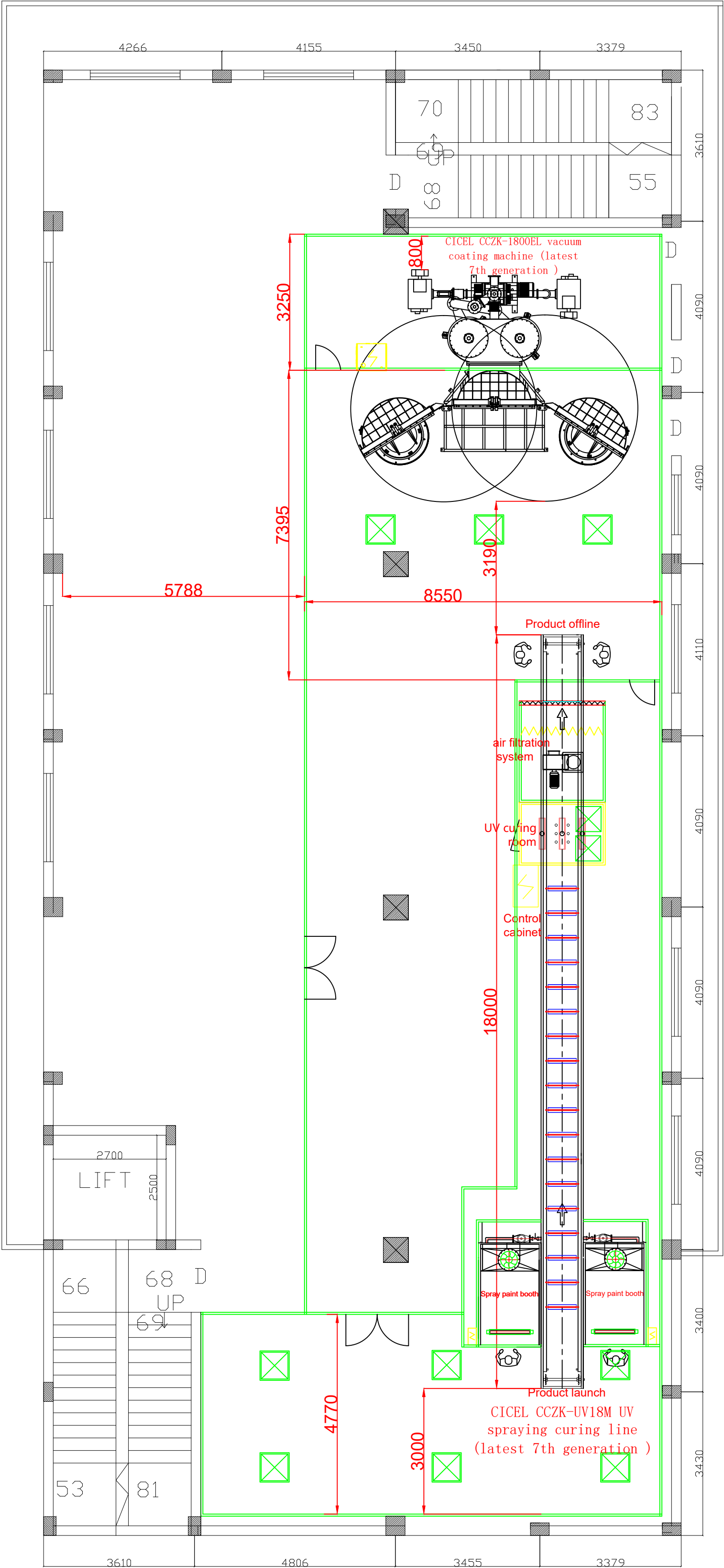
SECOND FLOOR PLAN NORTH ← (H=14')
