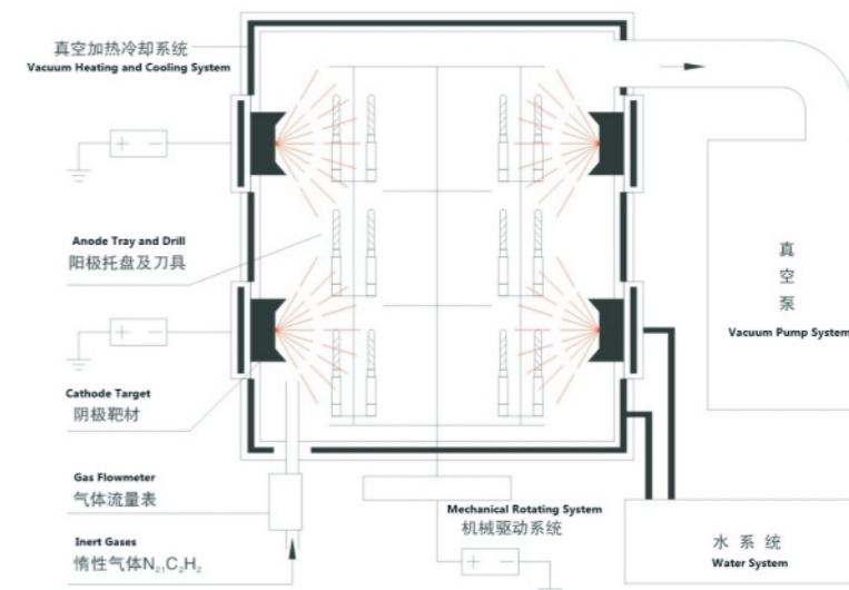
> 驰诚多弧离子工具镀膜系统 < CICEL multi-arc ion coating system (for tools coating)
