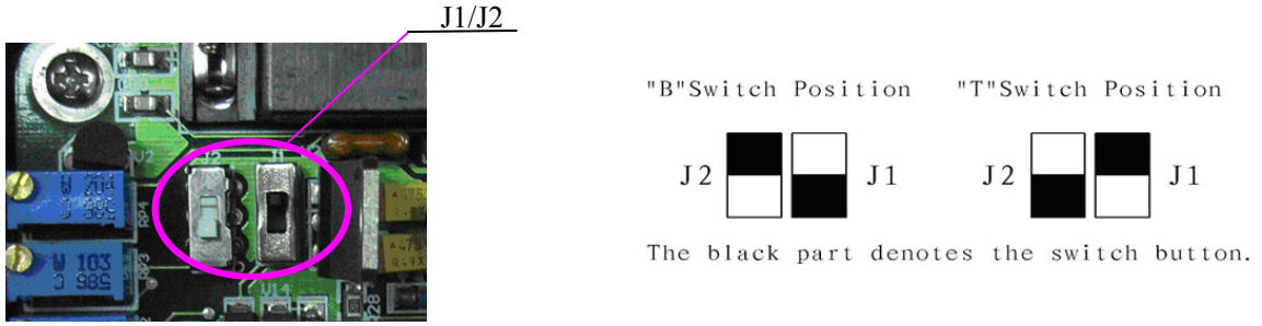
Figure 8. D07-19B MFC Socket Switch Connection
