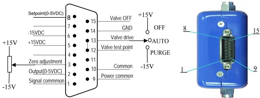
Figure 9. D07-19B MFC "T" Connection
