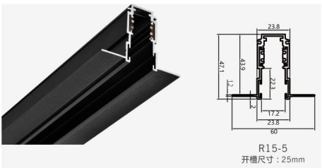
M15-R15-5 Size: L1000*W60*H47.1mm
