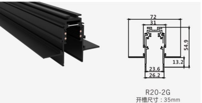
R20-2G Size : 31X53X72mm
