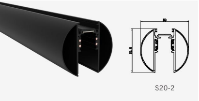
S20-2 Size : 59X53.6X59mm
