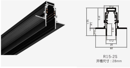
M15-R15-2S Size: L1000*W60*H52.1mm
