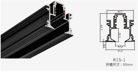
M15-R15-1 Size: L1000*W47.7*H47.7mm
