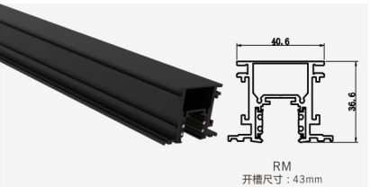
RM Size : 40.6X36.6X48.8
