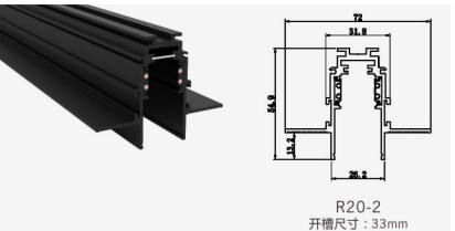
R20-2 Size : 72X54.9X26.3mm
