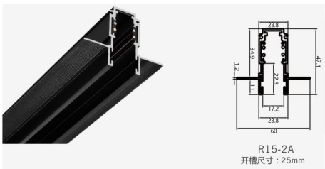
M15-R15-2A Size: L1000*W60*H47.1mm
