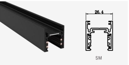
SM Size : 26.4X26.4X26.4mm
