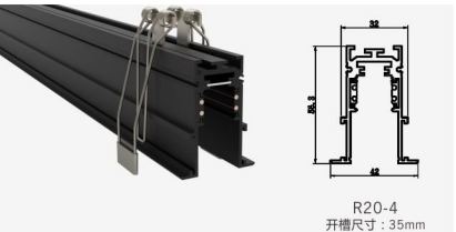
R20-4 Size : 32X56.3X42mm
