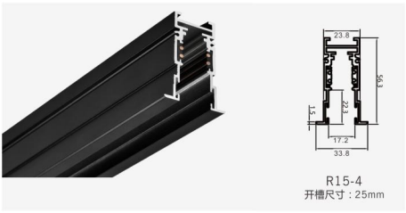
M15-R15-4 Size: L1000*W33.8*H56.3mm
