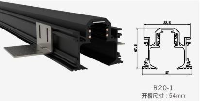
R20-1 Size : 53.5X47.3X57mm
