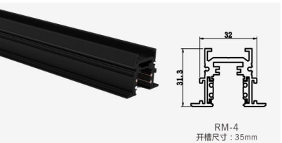
RM-4 Size : 31.3X32X42
