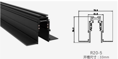
R20-5 Size : 70.9X54.9X31.8mm
