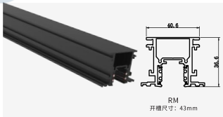
RM Size:40.6X36.6X48.8mm
