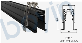
R20-4 Size:32X56.3X42mm
