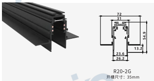
R20-2G Size:31X53X72mm
