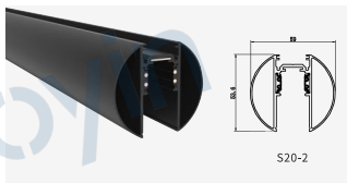
S20-2 Size:59X53.6X59mm
