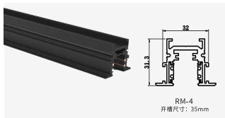
RM-4 Size:31.3X32X42mm
