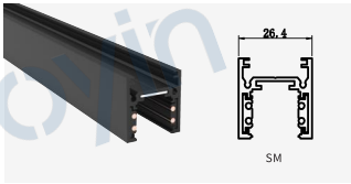
SM Size:26.4X26.4X26.4mm
