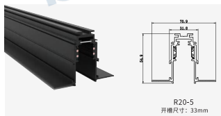
R20-5 Size:70.9X54.9X31.8mm
