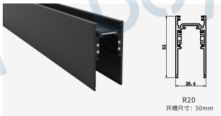
S20 Size:26.4X78.4X26.4mm
