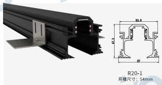
R20-1 Size:53.5X47.3X57mm
