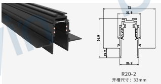
R20-2 Size:72X54.9X26.3mm
