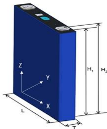
Fig.6 Diagram of LF150Cell direction
