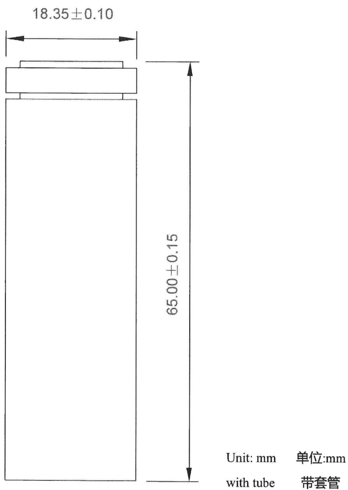
Fig. 1. Outline Dimensions of ICR18650/26V
