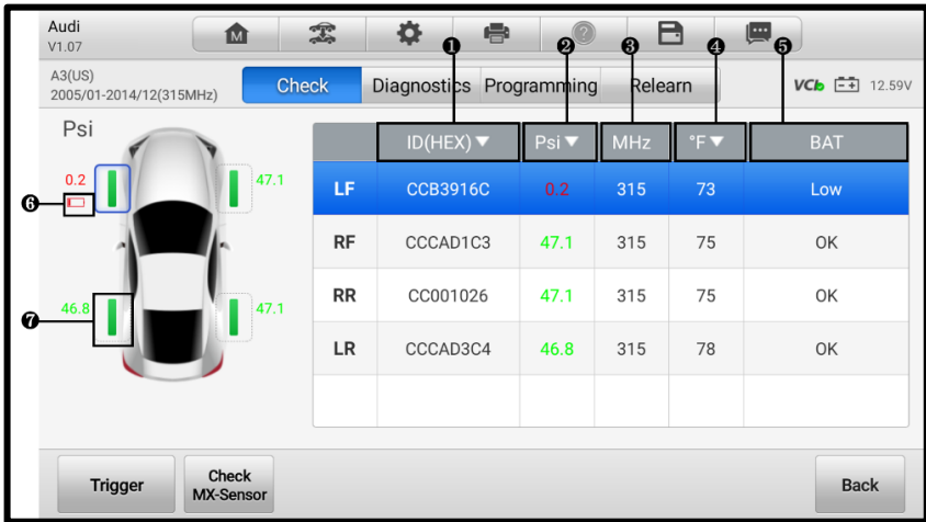
Figure 6-9 Check Screen
