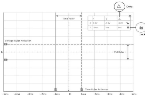
Figure 18-8 Measurement Rulers Display
