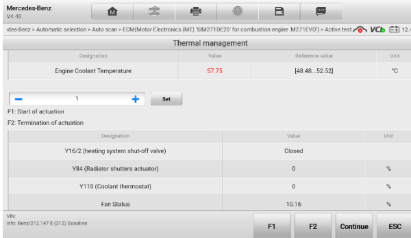
Figure 4-14 Active Test Screen
