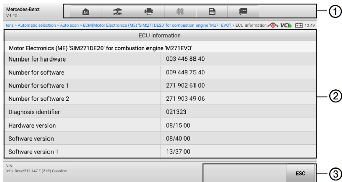
Figure 4-8 ECU Information Screen
