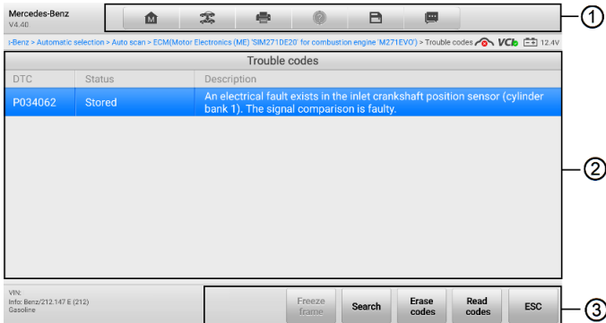
Figure 4-9 Read Codes Screen
