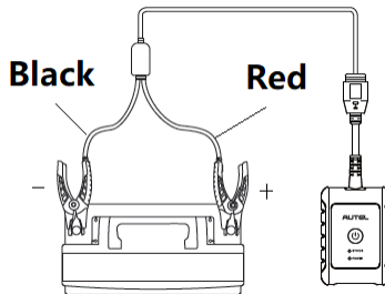
Figure 8-2 Connecting to a Battery
