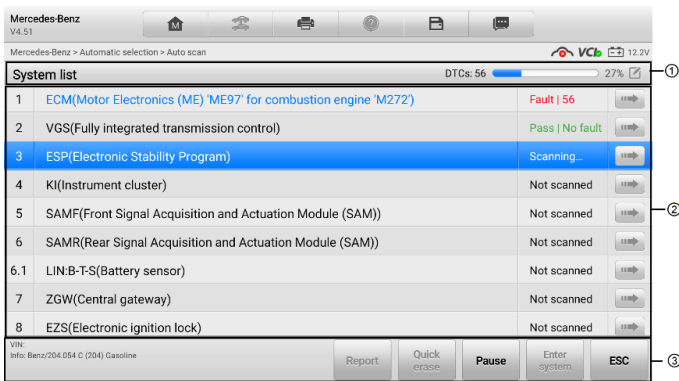
Figure 4-6 Auto Scan Operation Screen
