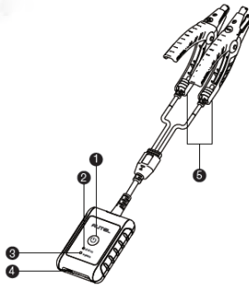
Figure 8-1 MaxiBAS BT506 Tester
