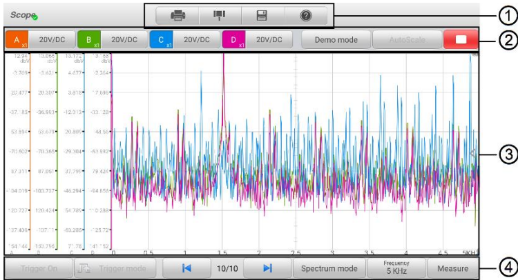
Figure 18-4 Oscilloscope Application Screen Layout
