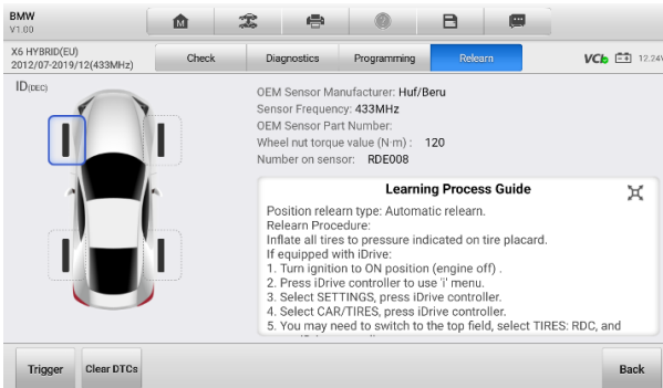
Figure 5-6 Relearn Function Main Screen
