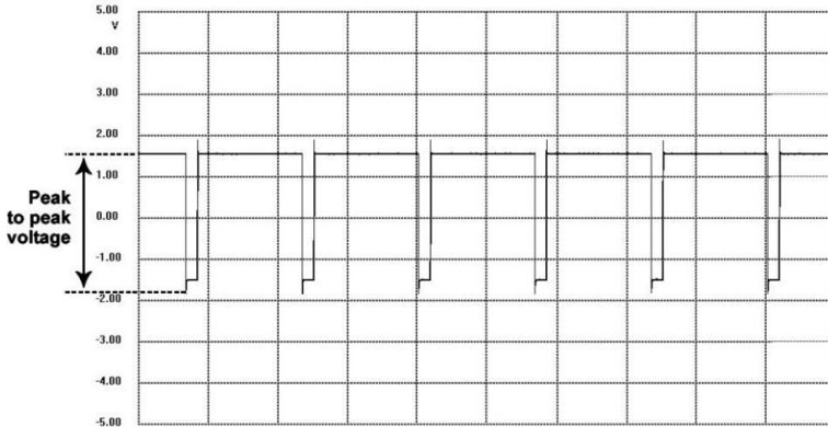
Figure 18-2 Square Waveform
