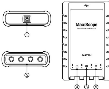
Figure 18-3 MaxiScope Front, Rear, and Top View
