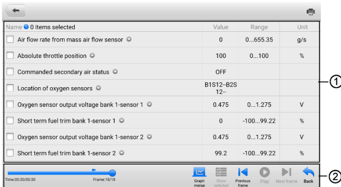
Figure 9-6 Data Playback Screen
