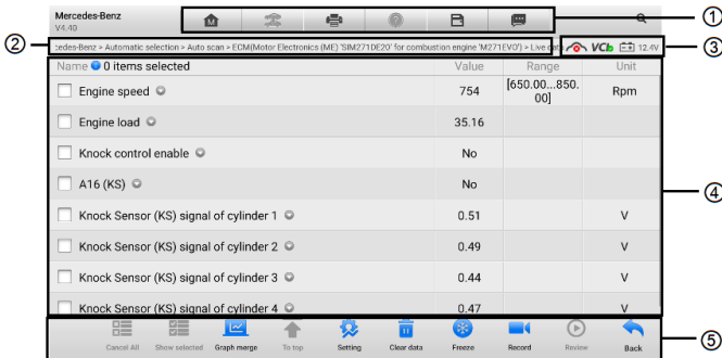
Figure 4-10 Live Data Screen
