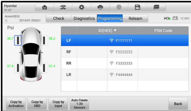
Figure 6-18 Programming Screen 2
