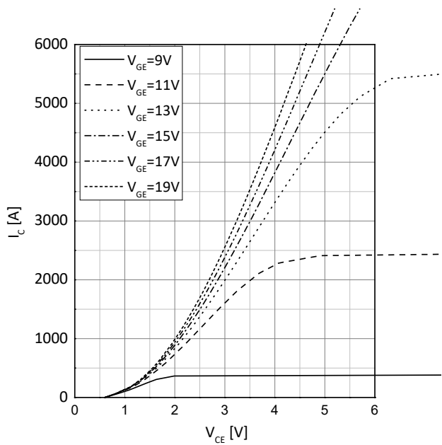
输出特性典型曲线 Typical output characteristics,chip level I_c=f(V_{ce}), T_{vj}=125^\circ\text{C}
