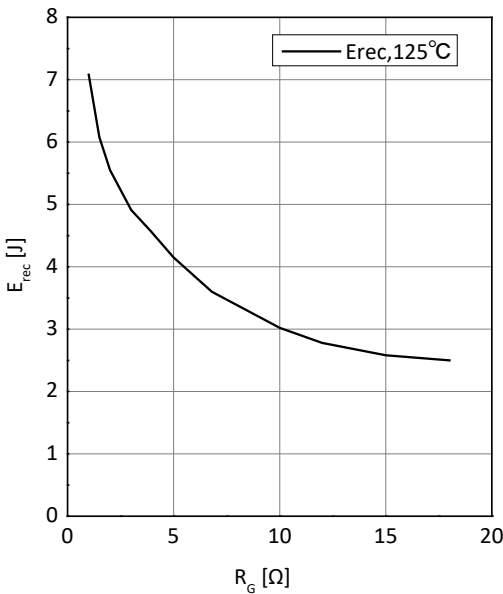
反向恢复损耗与门极电阻的关系曲线 Typical switching energies per pulse vs. gate resistor
