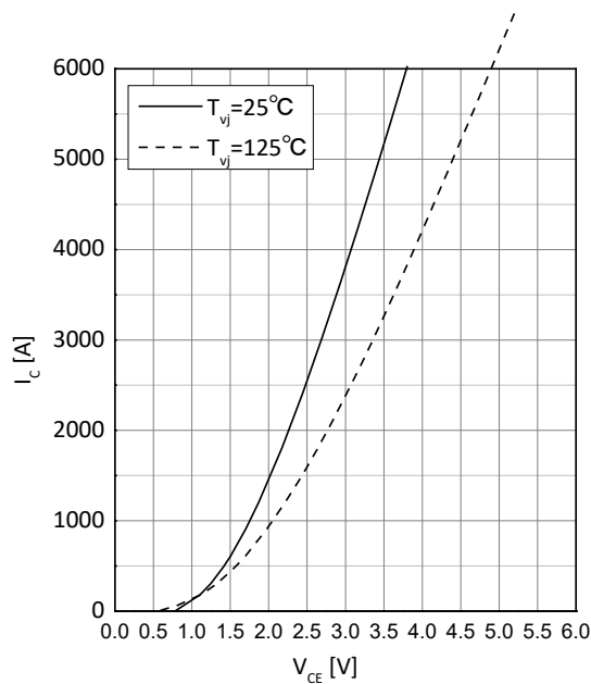
输出特性典型曲线 Typical output characteristics,chip level I_c=f(V_{ce}), T_{vj}=125^\circ\text{C}
