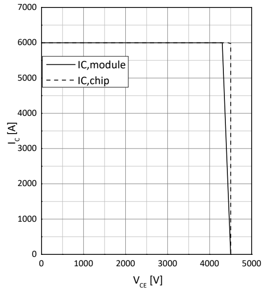
反偏安全工作区 Turn-off safe operating area (RBSOA) VGE=±15V, RGoff=6.8Ω, Tvj=125°C
