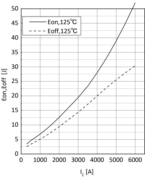
开关损耗 IGBT Switching losses IGBT E=f(I_c), V_{ge}=\pm 15\text{V}, R_{Gon}=1.5\Omega, R_{Goff}=6.8\Omega, C_{ge}=330\text{nF}, V_{ce}=2800\text{V}
