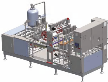
YSSH-1400 塑盒封口机 Plastic box sealer
