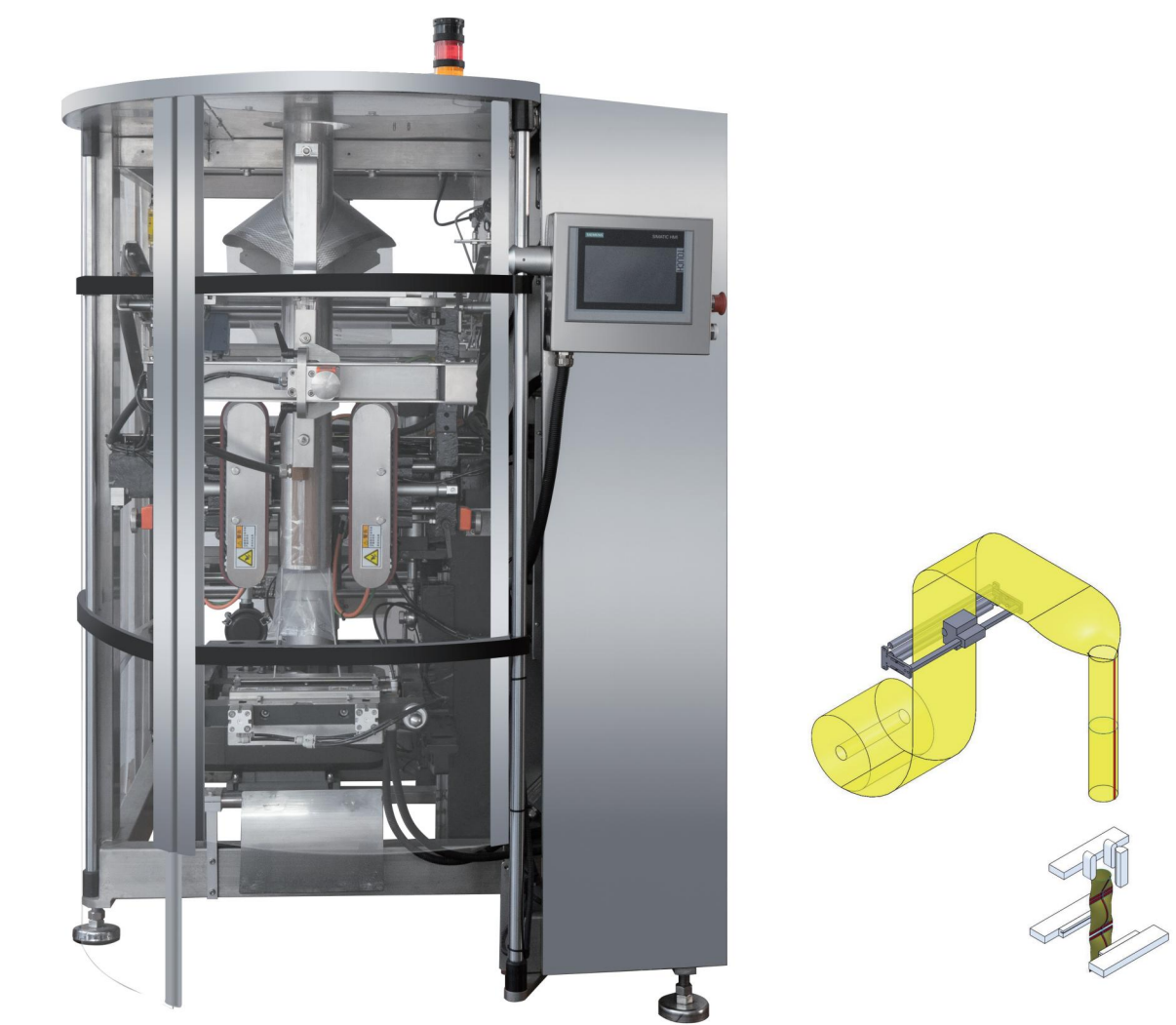
背封连续式立式机 (中小袋型/中大袋型) Back sealed, continuous machine (Small bag/Large bag)
