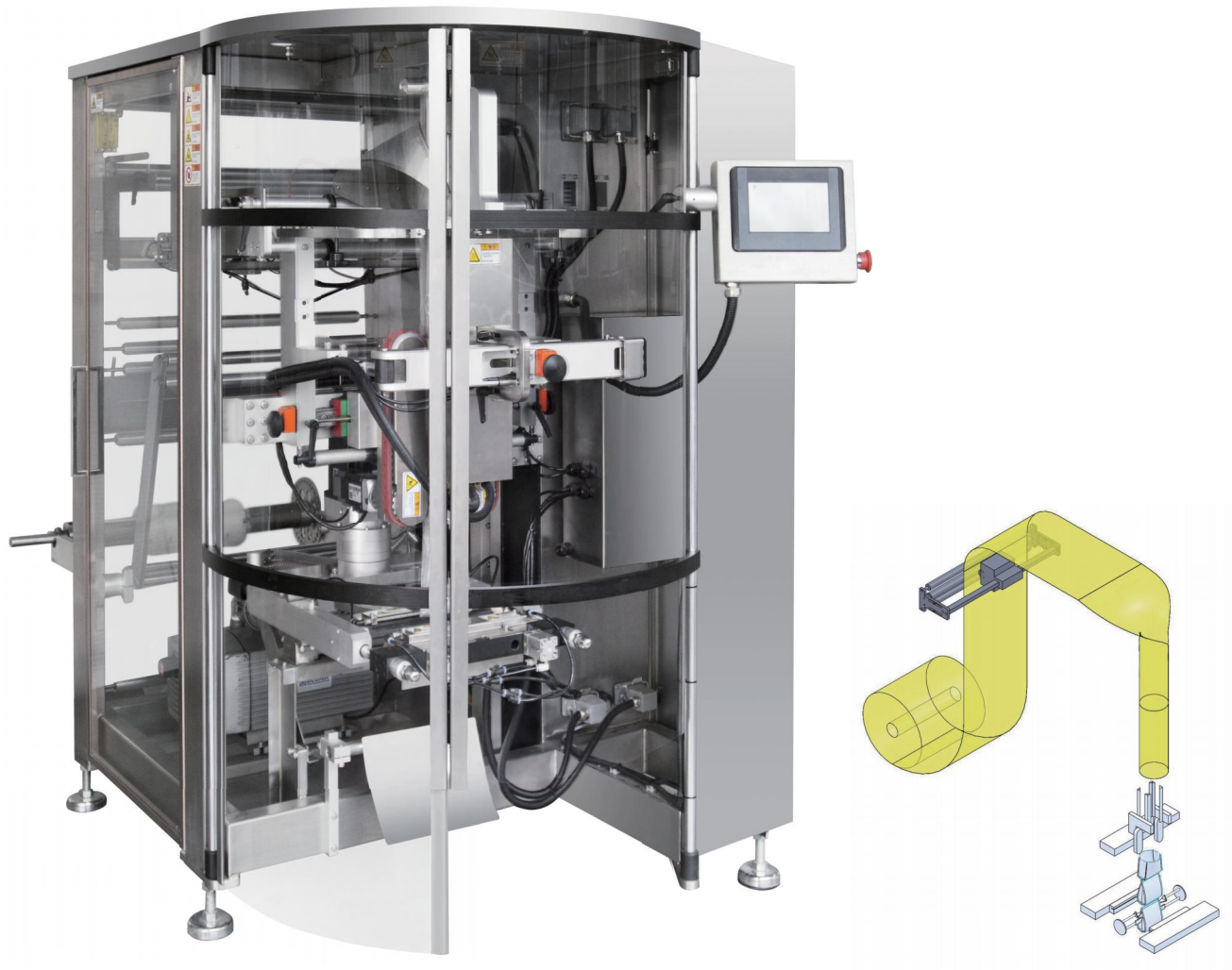
侧封烫边连续式立式机 (中小袋型/中大袋型) Corner sealed, quare heated, continuous machine (Small bag/Large bag)
