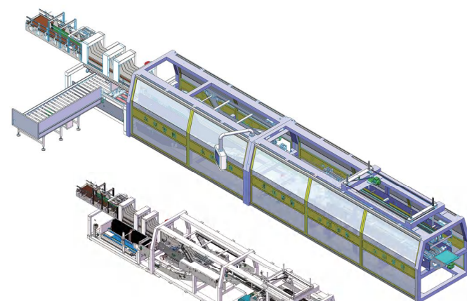
YS-ZX-60TA 纸包机 (同步带摩擦分纸片) wrap around case packer YS-ZX-60TB 纸包机 (立放纸板吸盘分纸片) wrap around case packer
