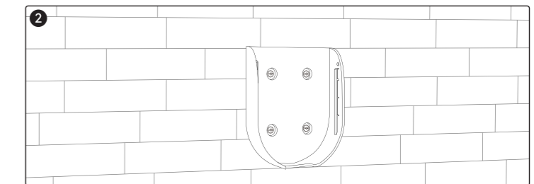
02. Use screws to attach the wall mount plate to the wall;
