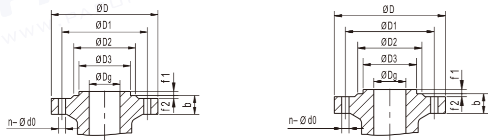
Inlet Flange
