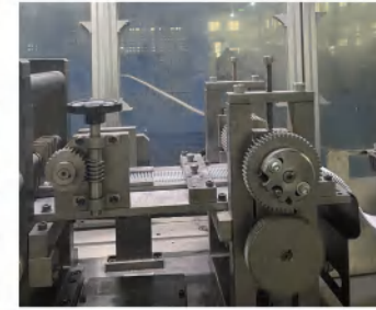
Aluminium Strip Fabrication
