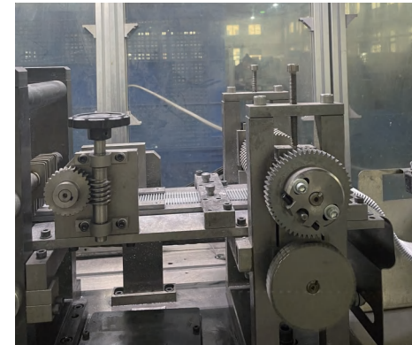
Aluminium Strip Fabrication
