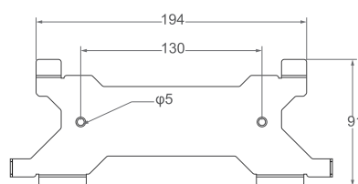
Mounting Bracket
