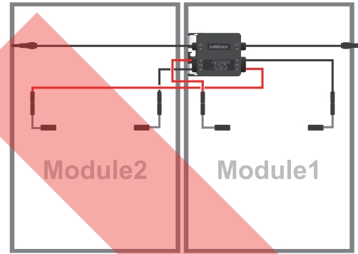
① Module1+ and Module2+ reversed
