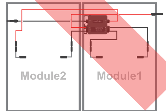
⑥ Module2+ and OUT- reversed
