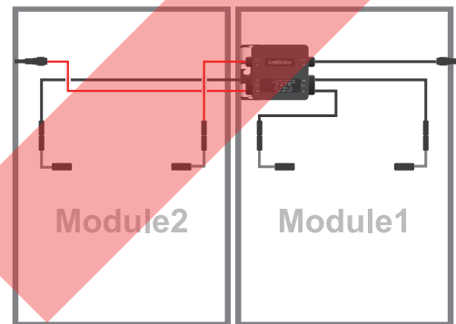
⑤ Module2- and OUT+ reversed
