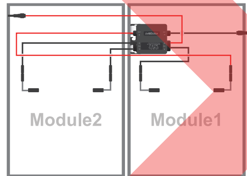
③ Module1- and OUT+ reversed
