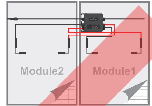
② Module1- and Module2- reversed
