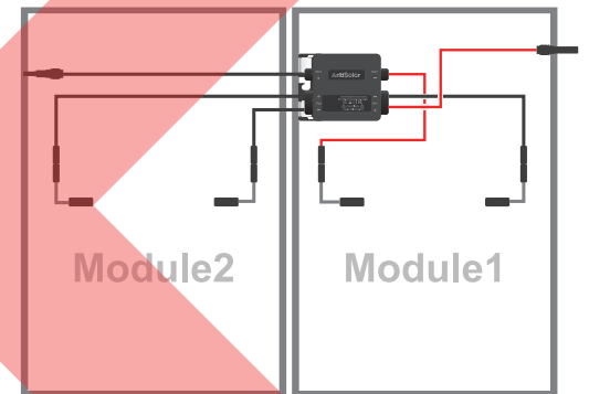
④ Module1+ and OUT- reversed
