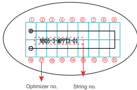
PV Array Wiring Diagram
