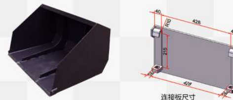
J33993-110 铲斗 J33993-110 BUCKET
