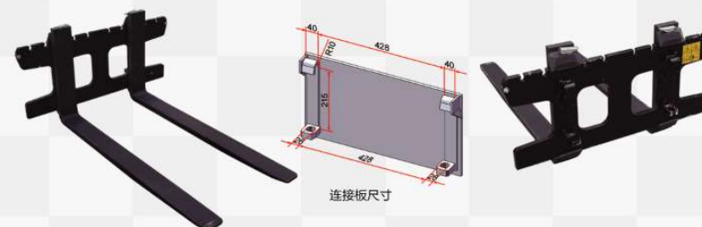
J21039 货叉 J21039 PALLET FORK
