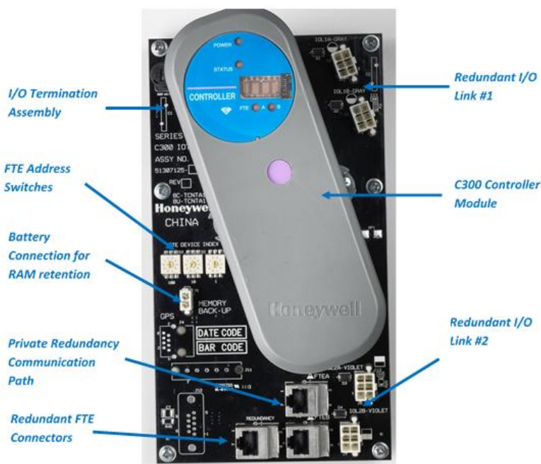
Figure 1 - C300 Controller
