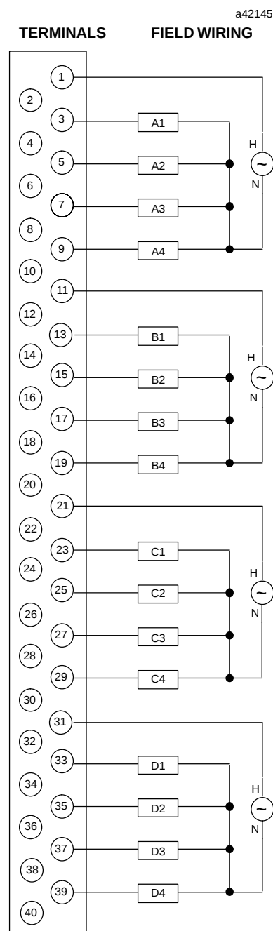
Figure 2. Field Wiring Connections
