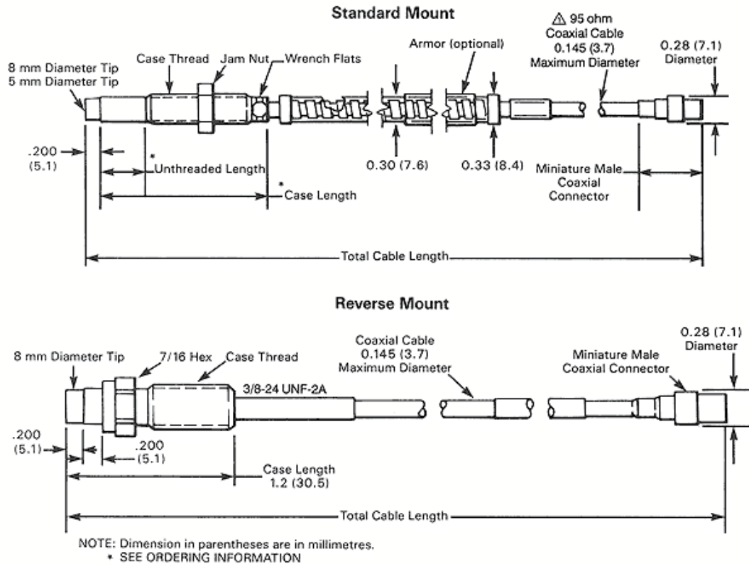
5 mm and 8 mm Proximity Probe Configurations
