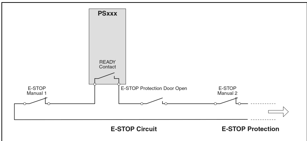
Figure 48: Power Supply READY Relay
