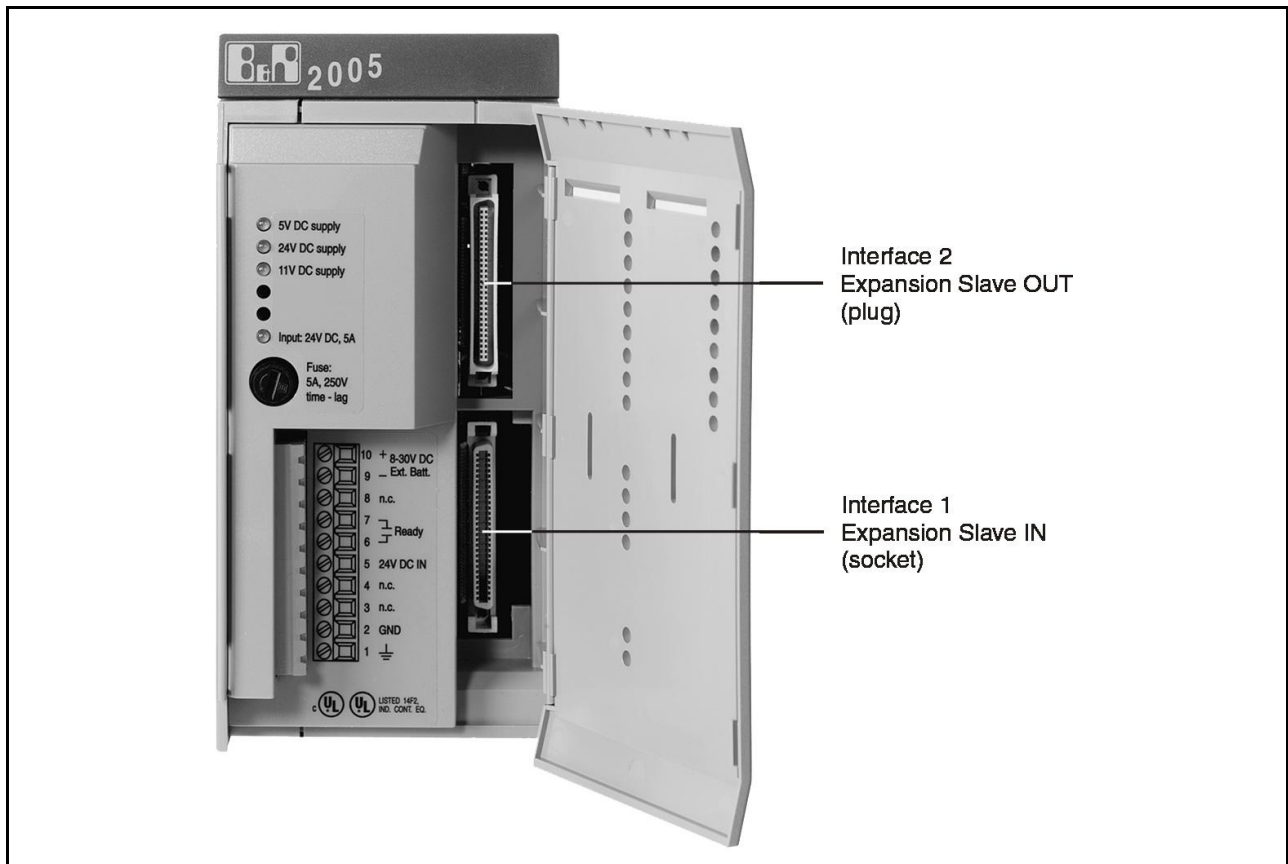
Figure 49: Power supply module interfaces for expansion slaves
