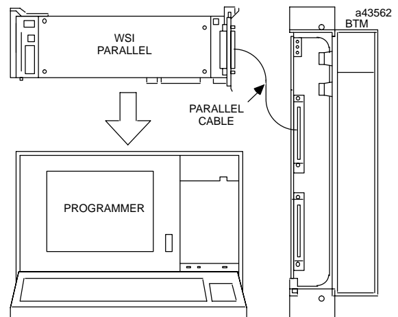
Figure 2. Parallel Programmer Attachment to BTM
