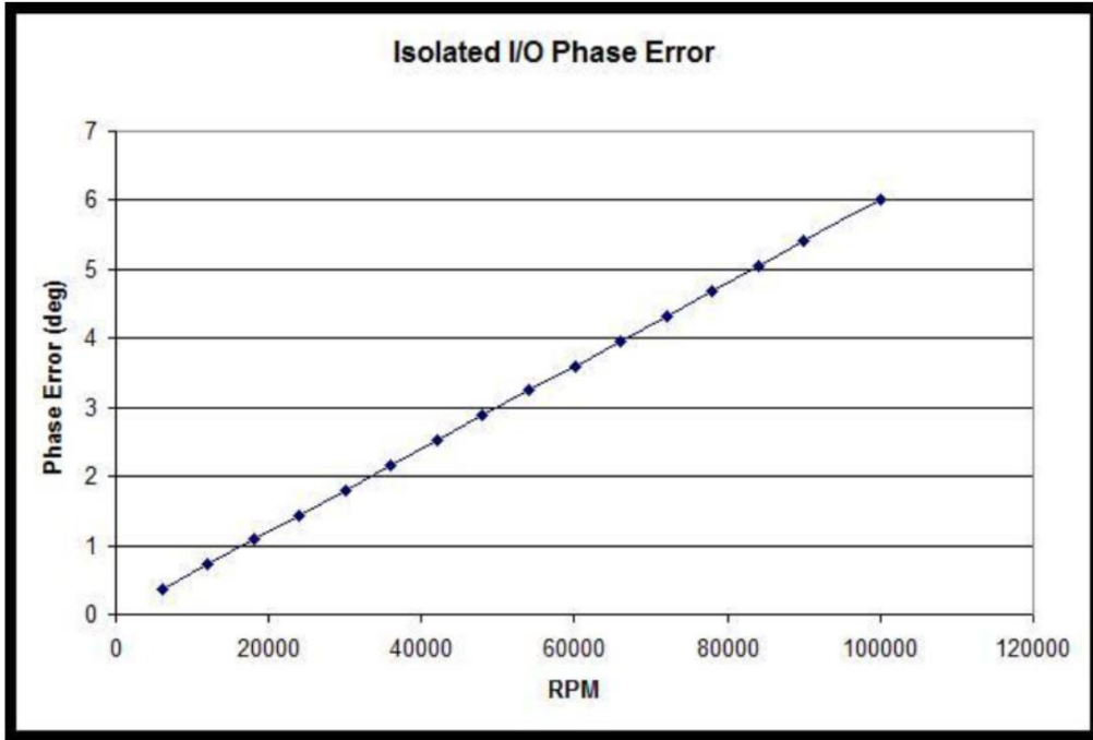
Figure 1: Phase Error vs. Machine Speed
