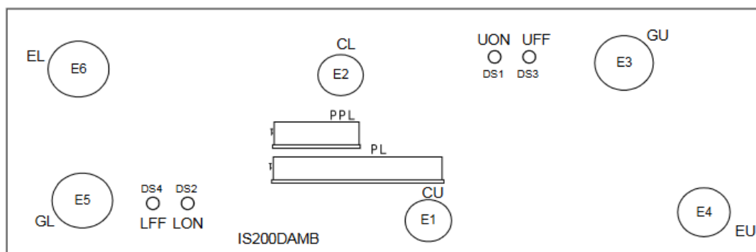
Figure 6. DAMB Board Layout Diagram
