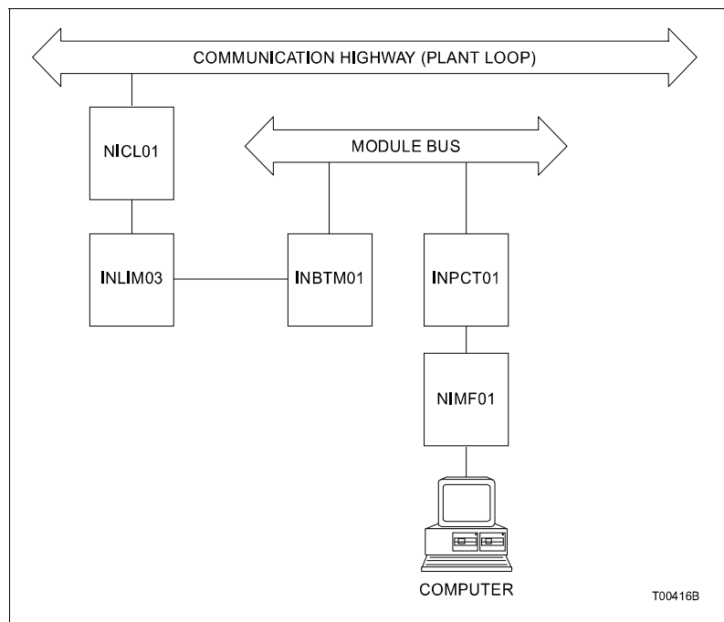
Figure 1-2. Example Plant Loop to Computer Interface Application
