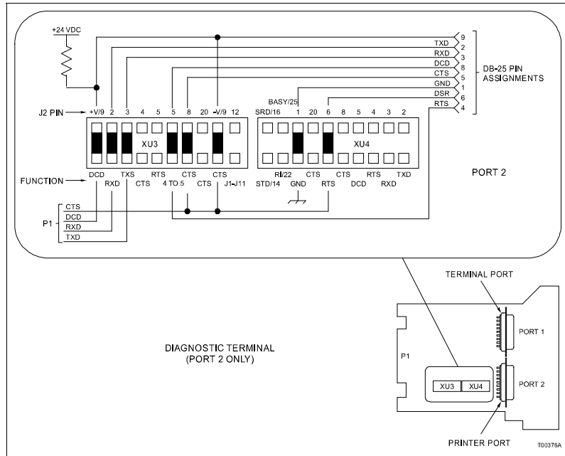
Figure 2-10. Dipshunt Configuration for Diagnostic Terminal (PPT module)
