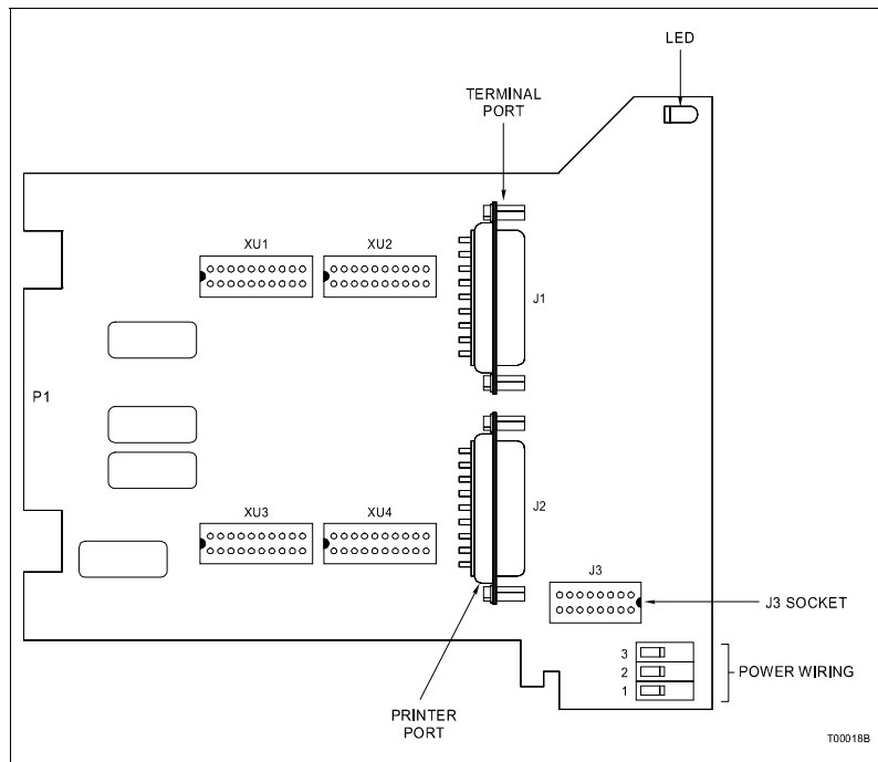
Figure 2-2. NIMF02 Connector Assignments and Dipshunt Locations
