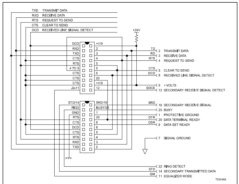
Figure 2-15. DB-25 Pin Assignments and RS-232-C Signals
