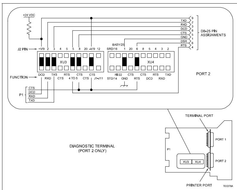
Figure 2-5. Dipshunt Configuration for Diagnostic Terminal (MFC and ICT modules)
