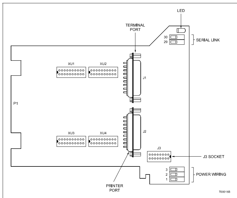
Figure 2-1. NIMF01 Connector Assignments and Dipshunt Locations
