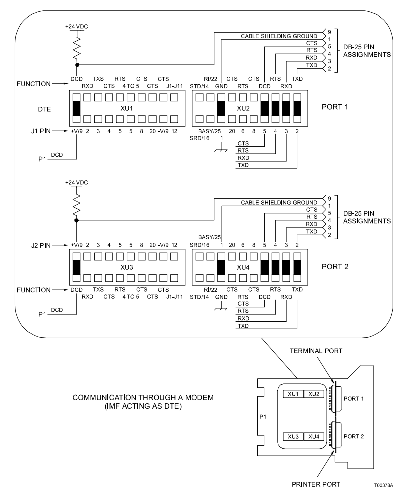
Figure 2-4. Dipshunt Configuration for Direct Connection to Modem (MFC and ICT modules)
