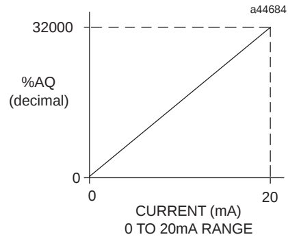
Figure 11-8. Scaling for Current Output, 0 to 20 mA
