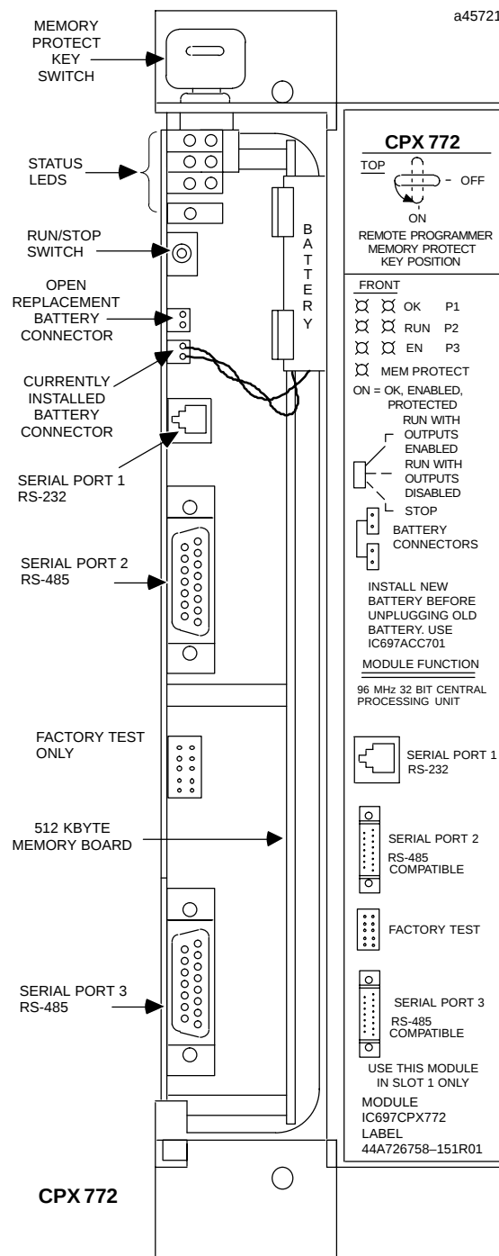
Figure 2. CPX 772 - Location of Major Features
